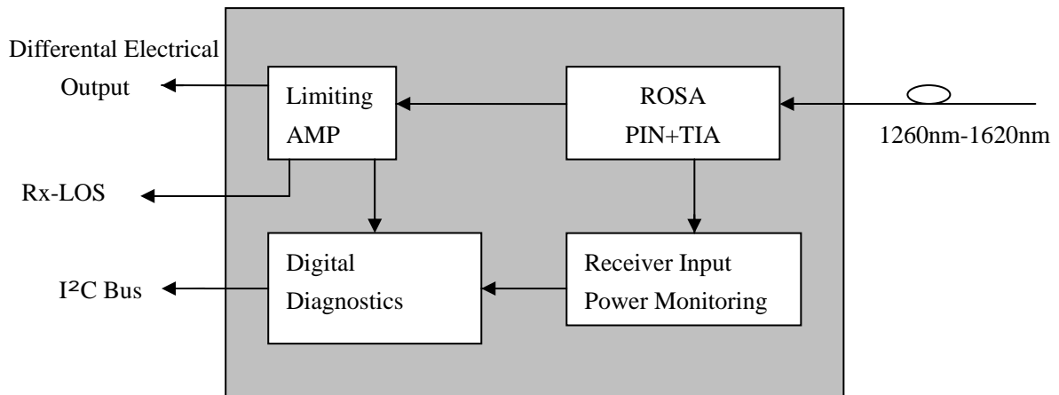
Figure 1: CRP13F5-11-SDI Functional Block Diagram
