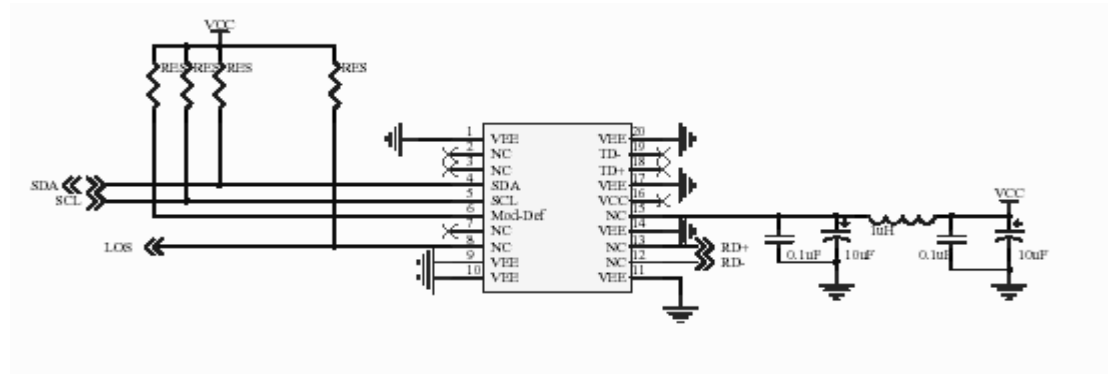
Figure 3: Recommended Circuit
