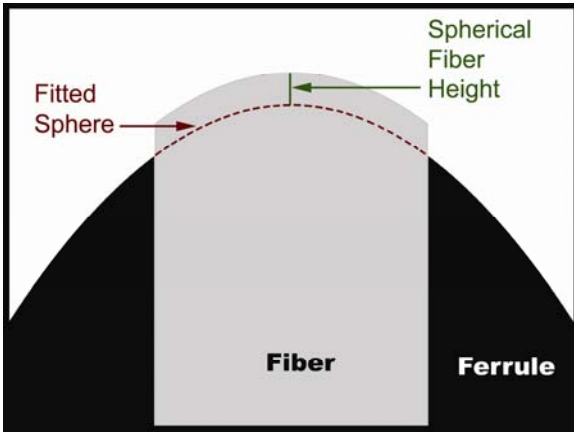
Radius = 25mm Spherical Fiber Height = +50nm
