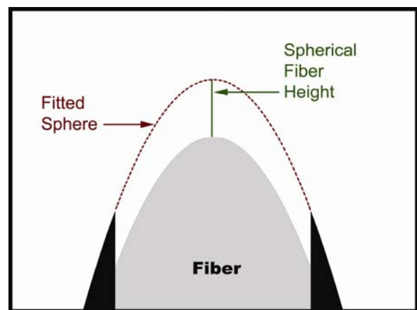
Radius = 7mm Spherical Fiber Height = -125nm
