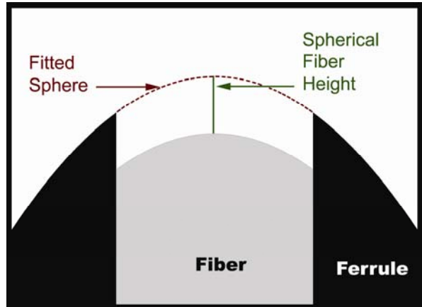
Radius = 25mm Spherical Fiber Height = -125nm
