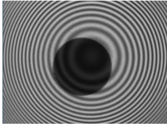
Interference Fringe Image of Connector Endfaces
