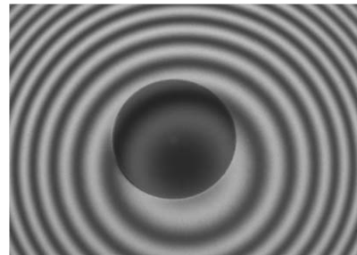
Circular Fringes from Interference between a Connector End and a Reference Mirror
