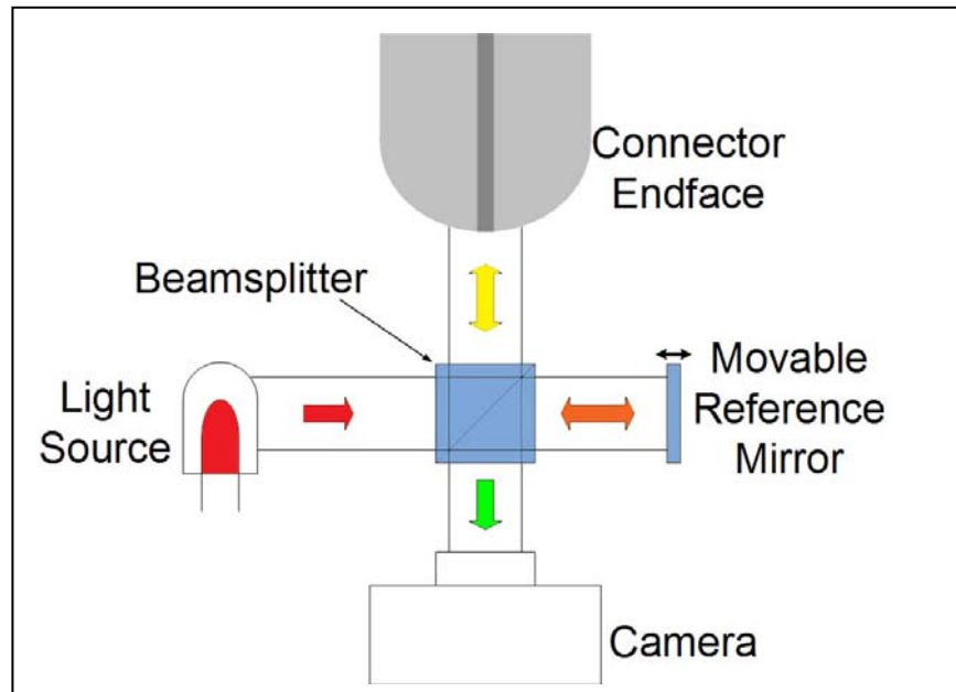
Michelson Interferometer
