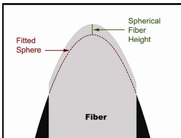
Radius = 7mm Spherical Fiber Height = +50nm
