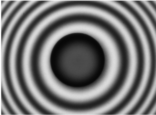
Interference Fringe Image of Connector Endfaces
