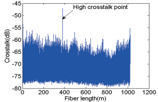
Figure 2. PM fiber quality inspection: Polarization x-talk measurement of 1000 m of raw fiber. High x-talk (-47 dB) is observed at 381 m.
