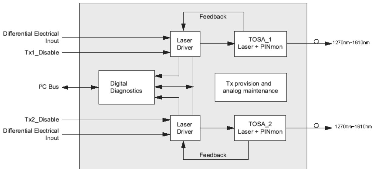
Figure 1: 2TPXXYYD6-11-SDI Functional Block Diagram
