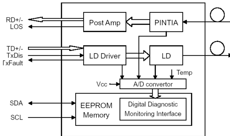
Figure 1: CSP15D6-11-SDI Functional Block Diagram
